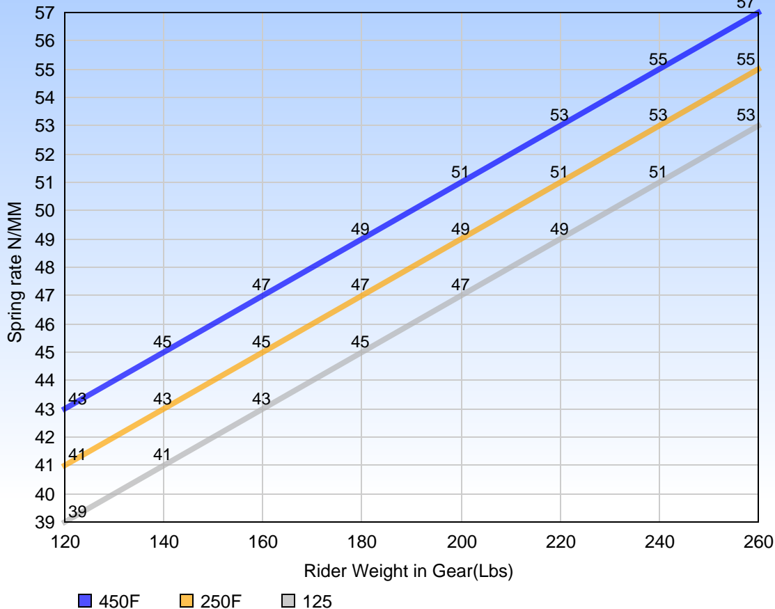
Spring rate Chart N2D 16 KTM Link
